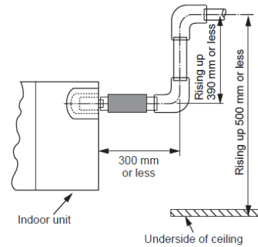
Drain upstanding size
